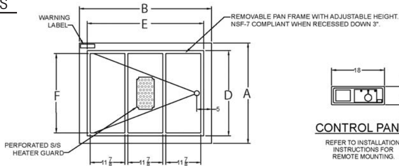
PLAN VIEW
