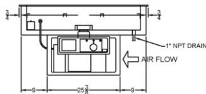
FRONT VIEW OPERATOR SIDE
