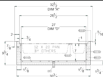
SECTION THRU
