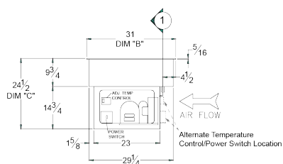
ELEVATION "A"
